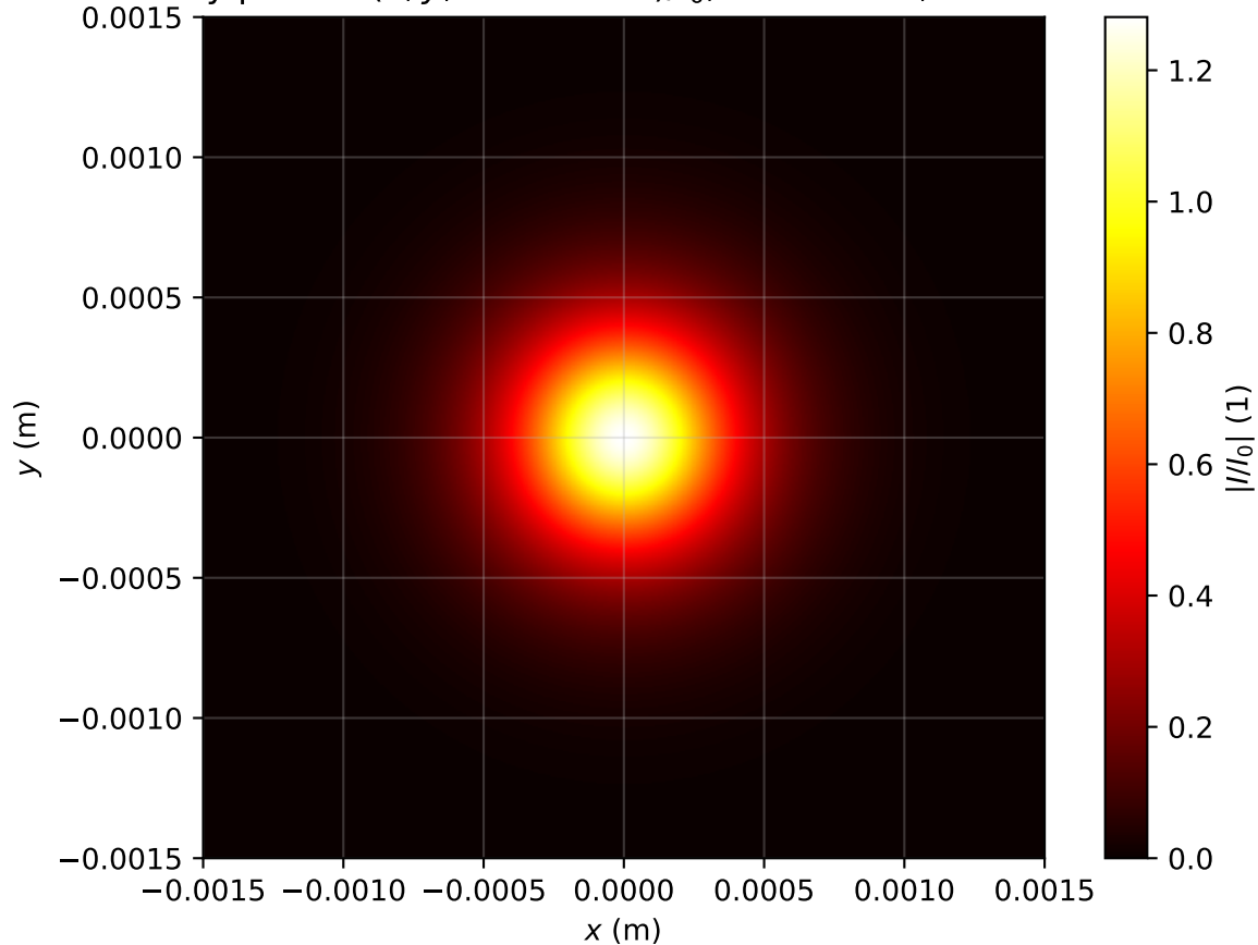
Intensity profile I(x, y, z = 0.955m)/I_0 , Pin=0.8Pcr, artificial time
